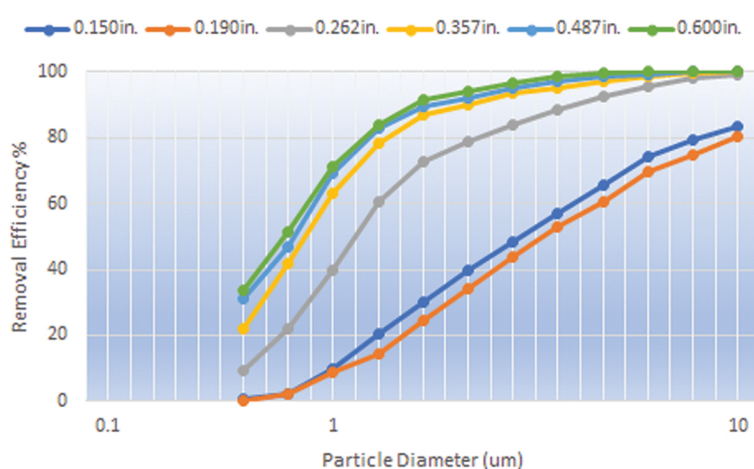
2" Fractional Efficiency vs. Particle Diameter
