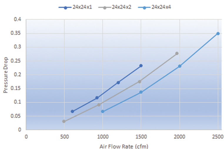
Initial Pressure Drop Vs. Air Flow Rate
