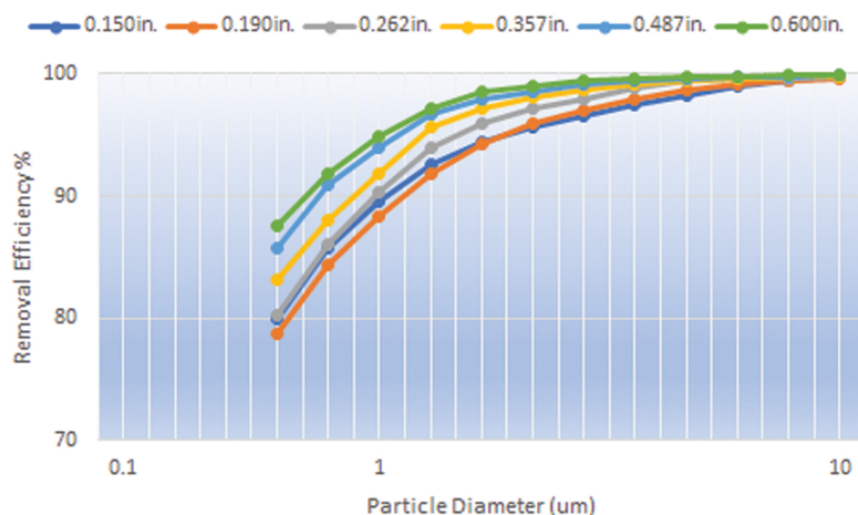
2" Fractional Efficiency vs. Particle Diameter
