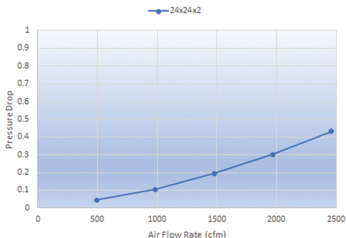
Pressure Drop Vs. Air Flow Rate
